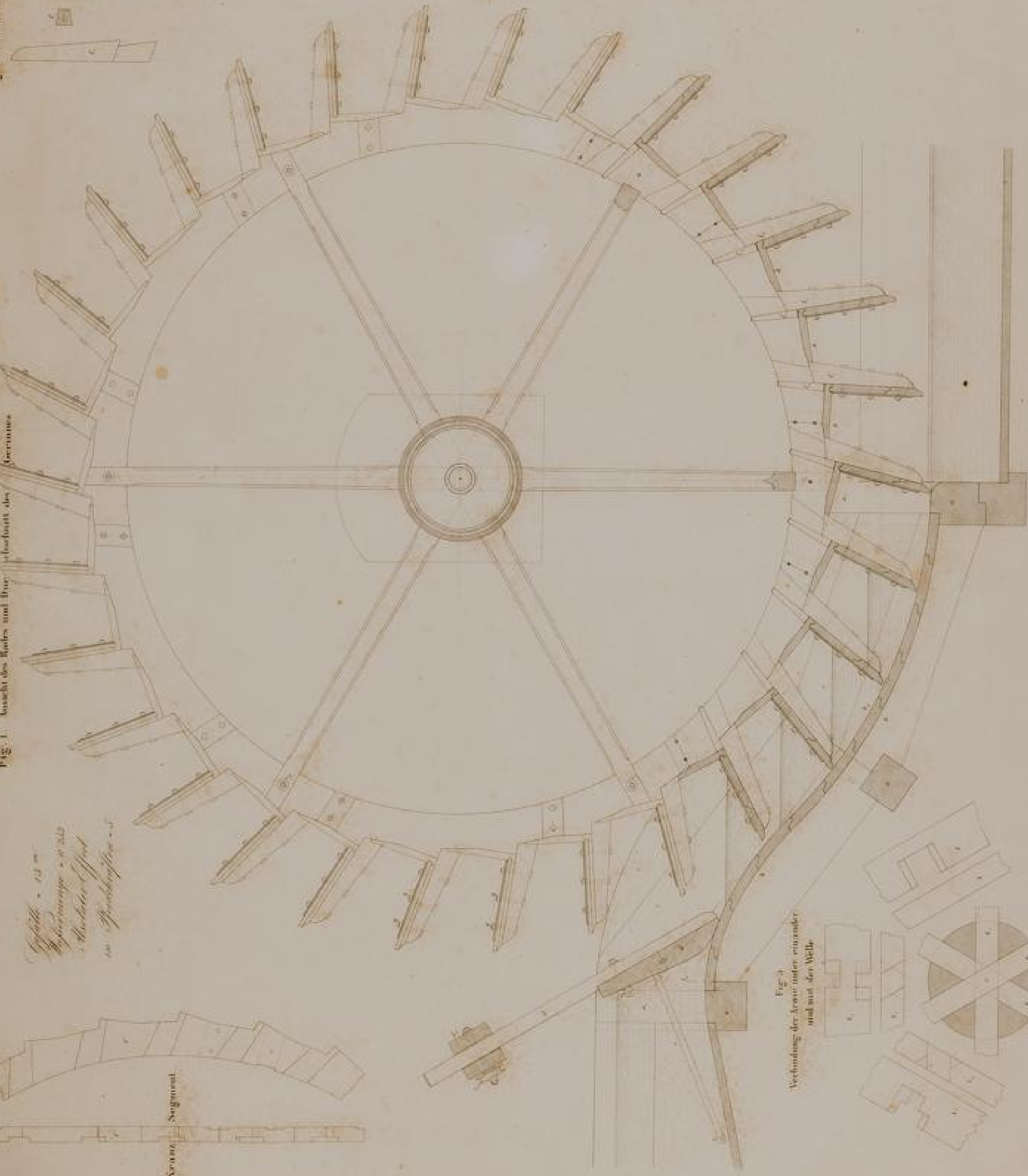
Fig. 5 Krone-Segment
